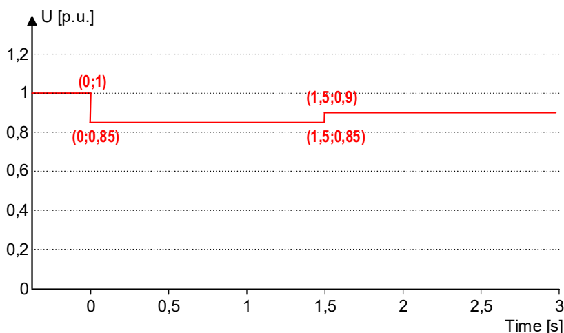
Figure 13 – Voltage-time profile for packup power systems
