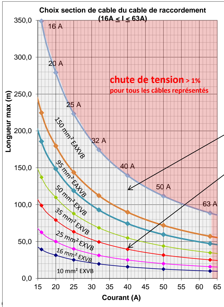
Figure 4.1 – Raccordement monophasé (2x230V ou 1N400)
