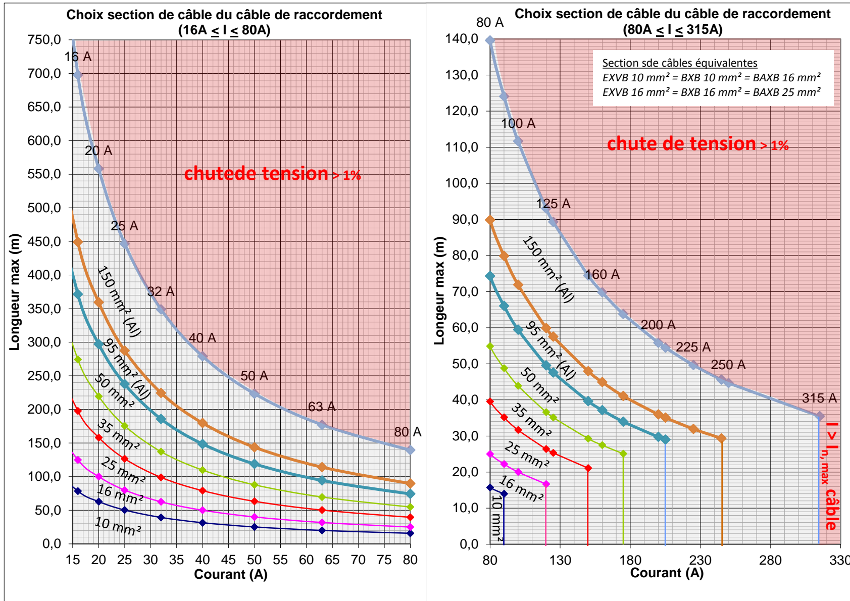
Figure 4.3 – Raccordement quadriolaire (3x400V+N)
